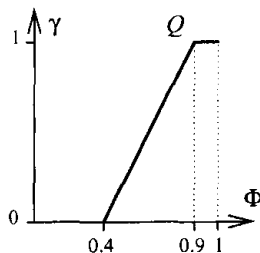
Fig. 2. Relative fuzzy quantifier "almost all": Q(\Phi) = 0 \leftrightarrow \Phi < 0.4 , Q(\Phi) = 1 \leftrightarrow \Phi > 0.9 and Q(\Phi) = 2(\Phi - 0.4) \leftrightarrow \Phi \in [0.4, 0.9] .
