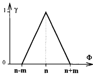
Fig. 1. Function "approximately n " ( n \pm m , where m is a margin).
