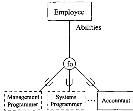
Fig. 10. Example 10: Fuzzy overlapping specialization.
