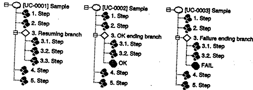
Fig. 5. Visual representation of conditional branches (evolved metamodel)
