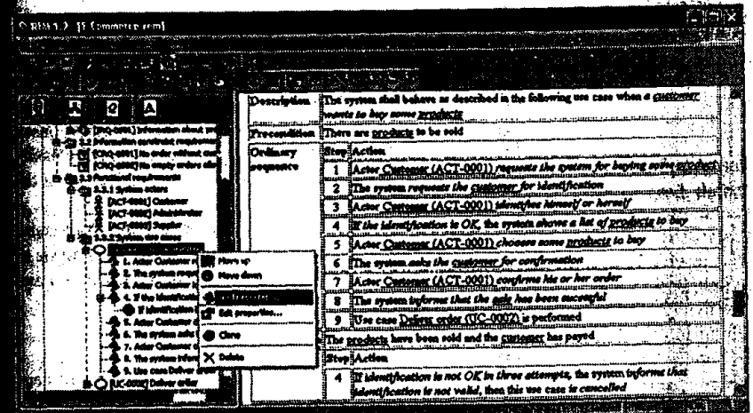
Fig. 2. REM user interface for use cases
