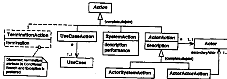
Fig. 7. Evolved metamodel for new specializations of actions
