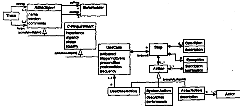
Fig. 1. Initial REM use case metamodel
