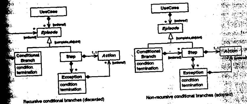
Fig. 4. Tentative evolved metamodels for conditional branches
