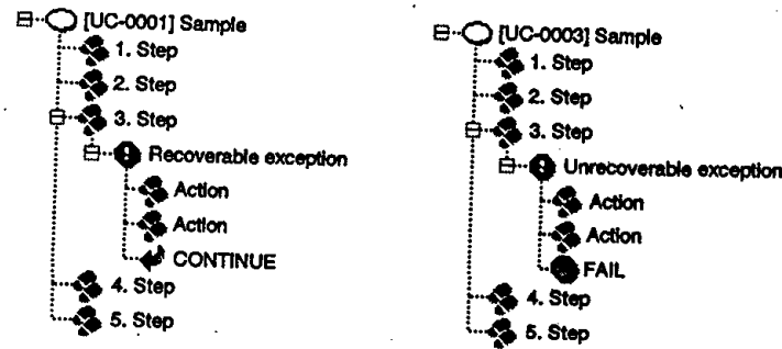
Fig. 6. Visual representation of exceptions (evolved metamodel)
