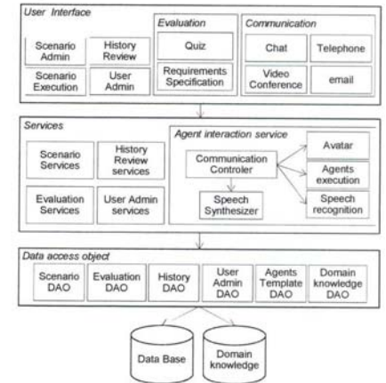
Figure 2. Architecture of the simulator.
