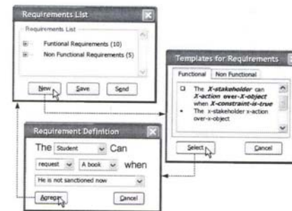
Figure 4. Prototype of requirements documentation interface
